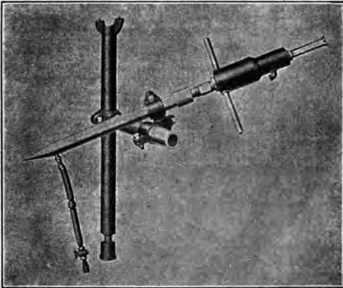
Fig. 30. Hardscoeg Wonder Air Hammer Drill on a Column.
